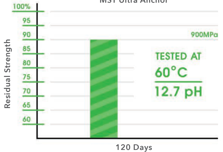
Alkali Resistance Testing of MST Ultra Anchor
